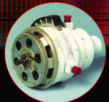
Generator A/C
