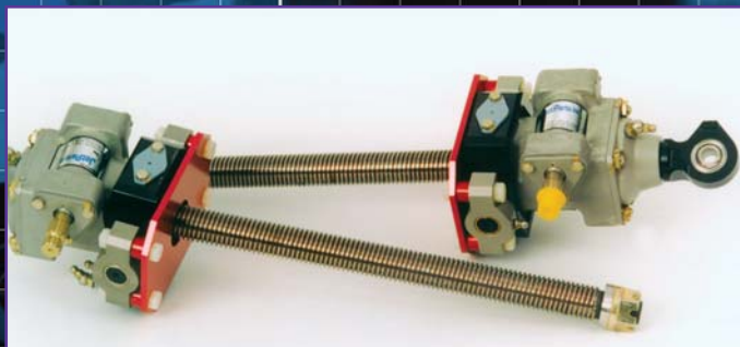
F50, F900 Screw Jacks
